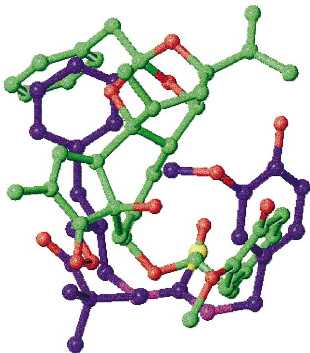
Figure 1. Superposition of 35 on resiniferatoxin.
